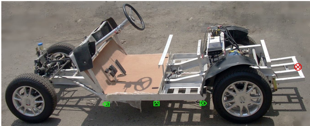
The California Roadster eGC chassis ( body removed ).
